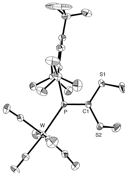
Fig. 3. An ORTEP drawing of 11 with 30% probability ellipsoids. Hydrogen atoms are omitted for clarity. Selected bond lengths ( \text{\AA} ) and angles ( ^{\circ} ): W–P 2.550(1), P–C1 1.687(6), P–Mes* 1.849(5), C1–S1 1.747(6), C1–S2 1.738(6), S1–CH 3 1.805(6), S2–CH 3 1.796(10), W–P–C1 124.2(2), W–P–Mes* 133.5(2), Mes*–P–C1 102.3(3), P–C1–S1 122.4(4), P–C1–S2 117.9(3), S1–C1–S2 119.8(3).
