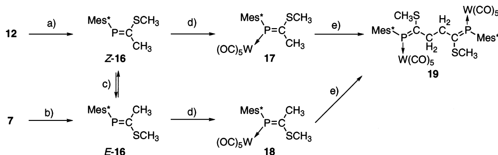
Scheme 5. Preparation of 2-methylsulfanyl-1-phosphapropenes. Reagents and conditions: a) (1) n -BuLi/THF/–78 °C, (2) (CH 3 S) 2 /–78 °C; b) (1) n -BuLi/THF/–78 °C, (2) CH 3 I/–78 °C; c) medium pressure Hg lamp (100 W)/benzene/5 °C/4 h; d) W(CO) 5 (thf); e) (1) n -BuLi/THF/–78 °C, (2) CuCl 2 /–78 °C.
