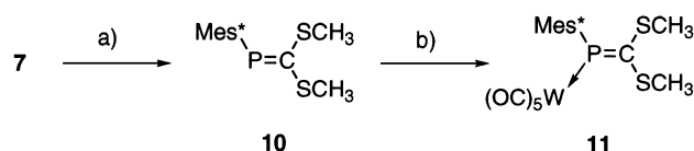
Scheme 3. Preparation of bis(methylsulfanyl)-substituted phosphoethenes. Reagents and conditions: a) (1) n -BuLi/THF/ -78^{\circ}\text{C} , (2) (\text{CH}_3\text{S})_2 / -78^{\circ}\text{C} ; b) \text{W}(\text{CO})_5(\text{thf}) .
